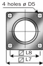
Rear Flange Mount - Fa
