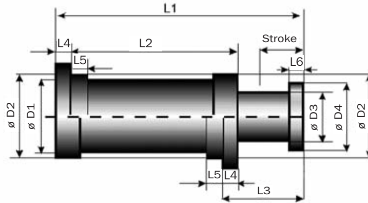
Front Flange Mount - Fc
