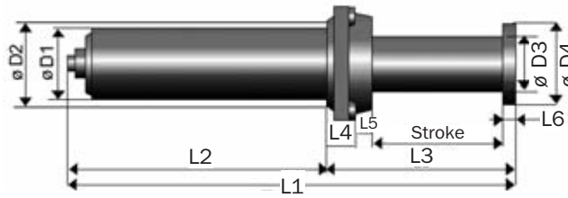
BCLR Series - Front Flange Mount- Fc
